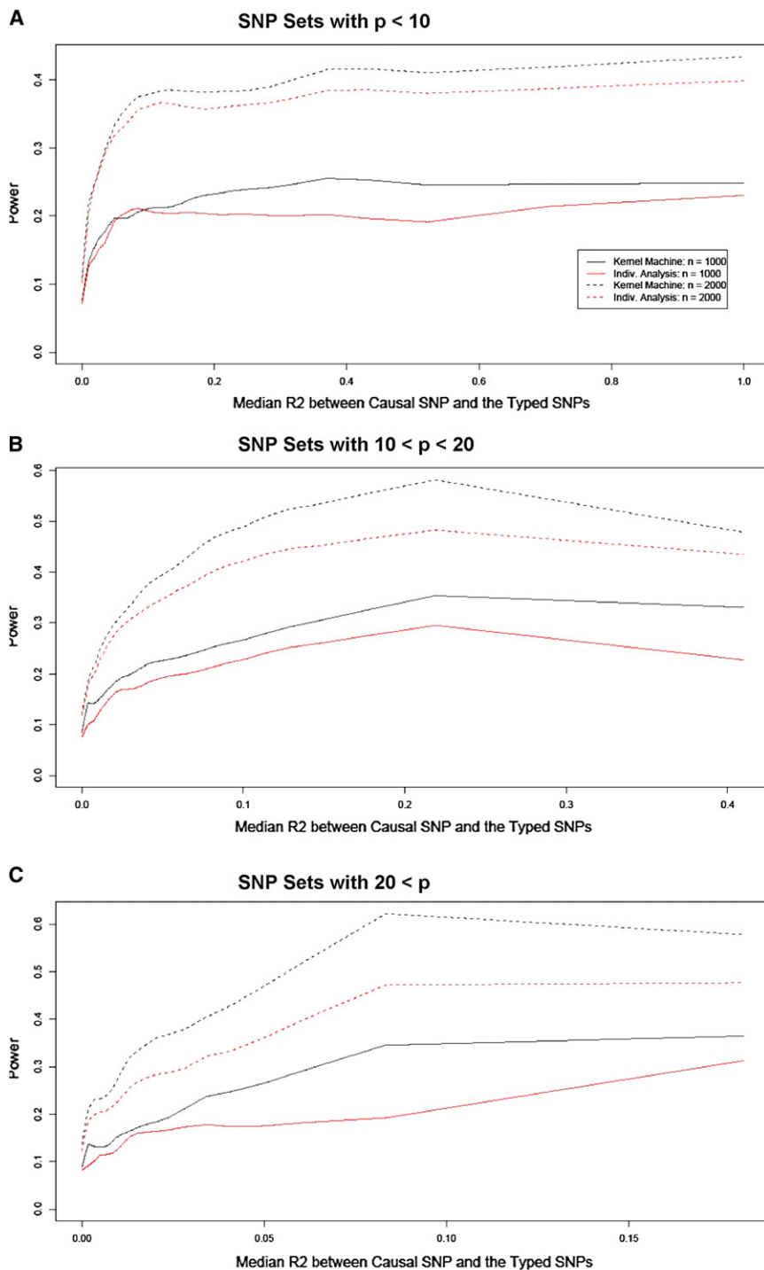
Figure 3. Smoothed Empirical Power Curves as a Function of Median R^2 between the Causal SNP and the Typed SNP for SNP Sets Based on a Range of Genes
