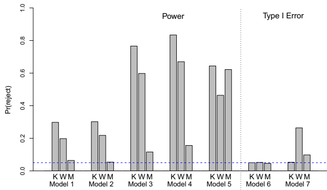
Figure 4. Comparison of the Power and Type I Error of the Logistic Kernel-Machine Test, the Wessel and Schork Method, and Mukhopadhyay et al.'s Approach
