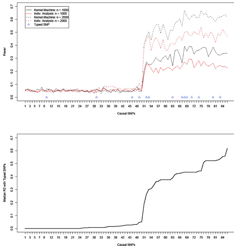
Figure 2. Empirical Power for SNP Sets Based on ASAH1
